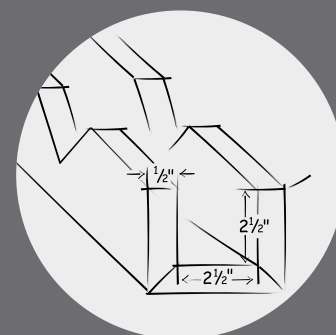
2 1/2" x 2 1/2" x 2 1/2" U-shape; 1/2" thick polyethylene foam; Double notch fits corner
