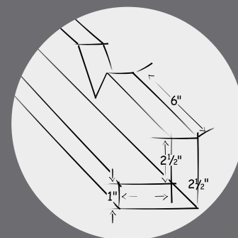
2 1/2" x 2 1/2" L-shape; 1" thick polyethylene foam; Precision notch fits corner
